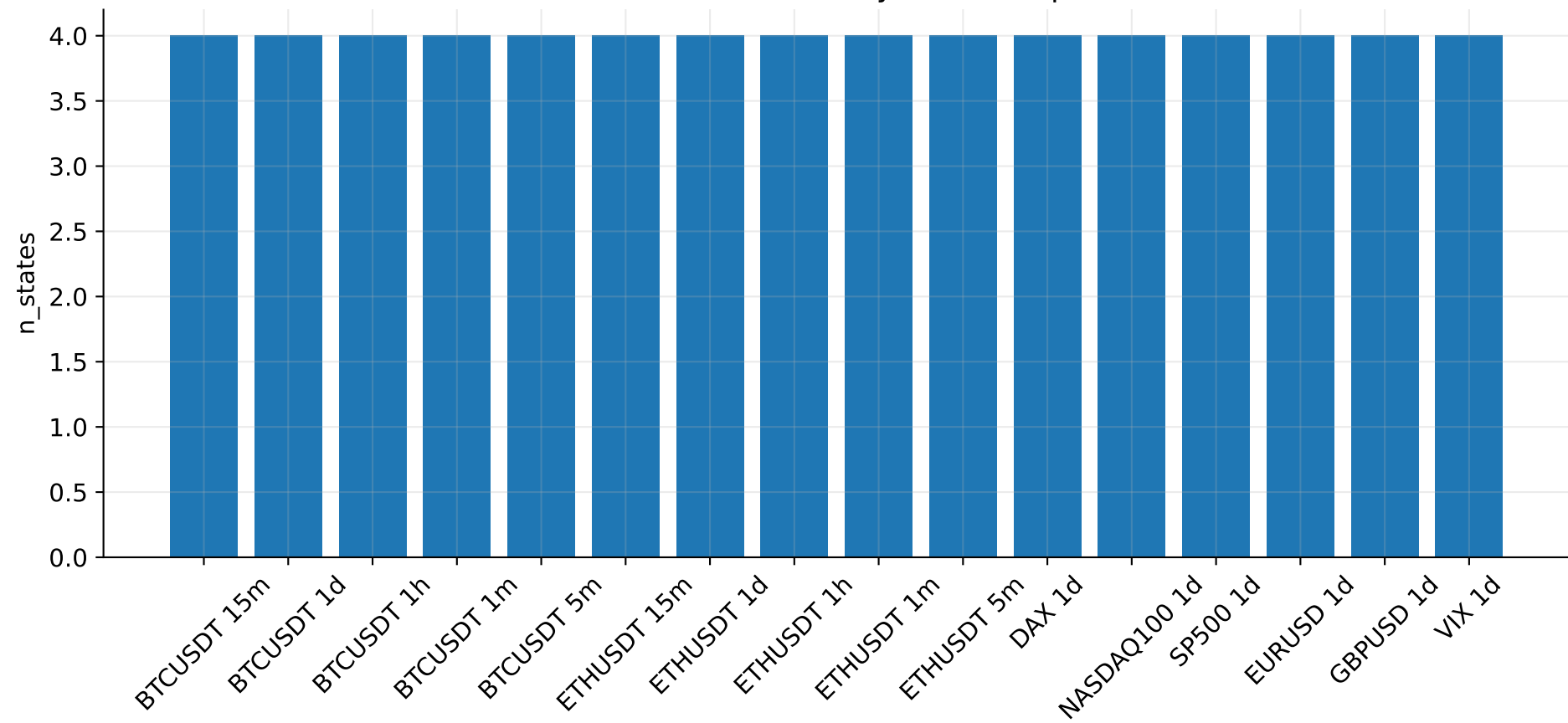
Selected HMM state count by thesis-scope dataset
